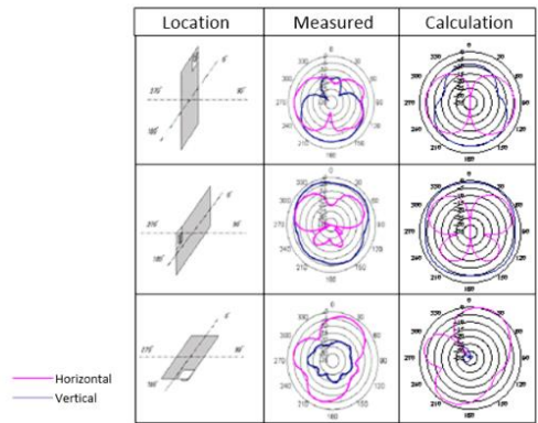
Directivity
