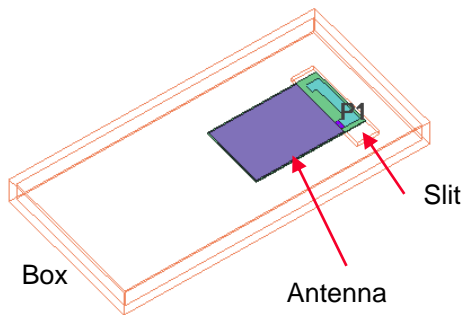
Antenna Model
